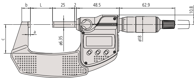
Ratchet stop type (up to 100mm/4")
