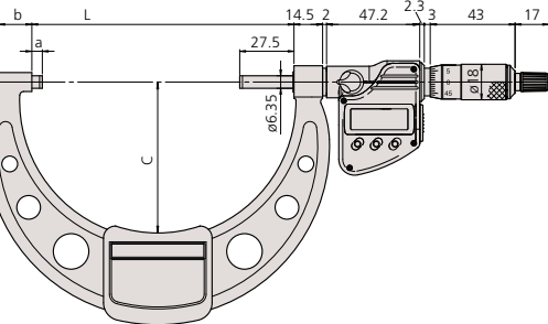
Ratchet stop type (over 100mm/4" to 300mm/12")
